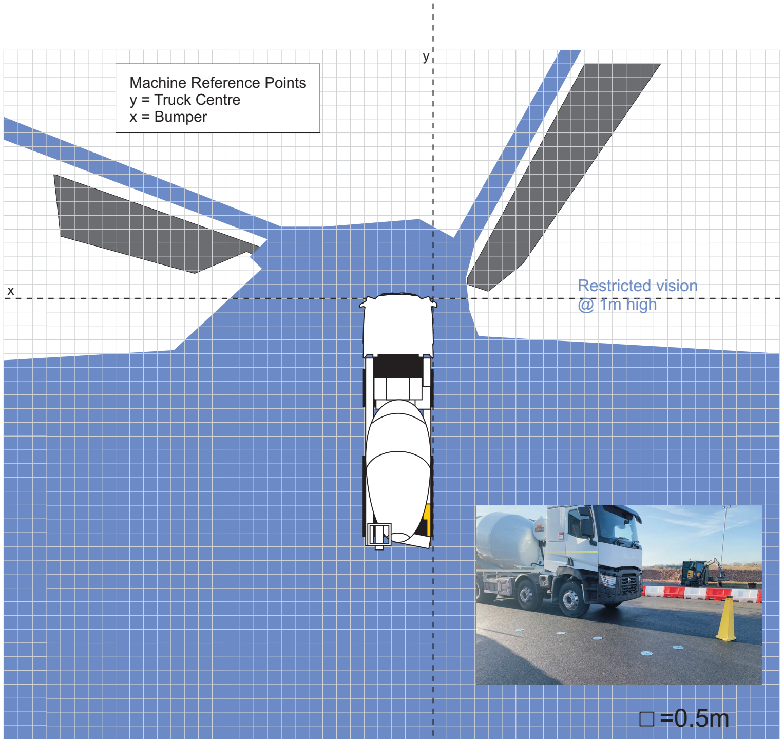
Renault 8x4 Mixer
