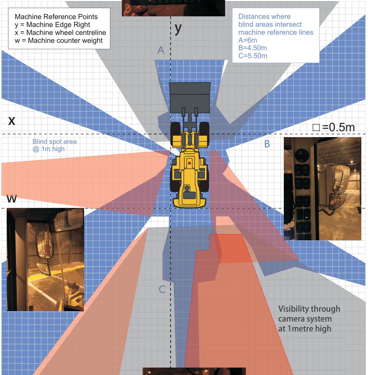
Volvo L150G
