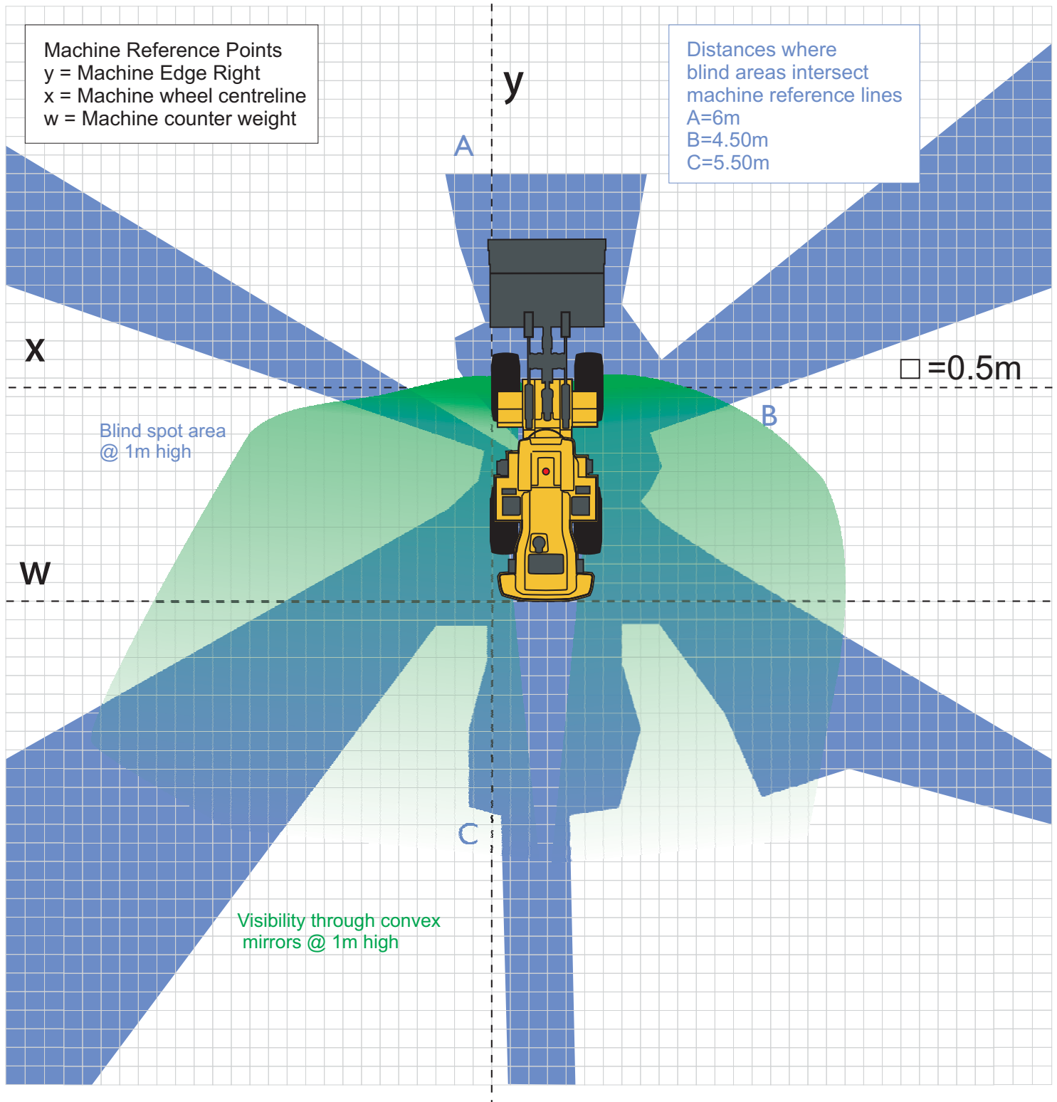
Volvo L150G
