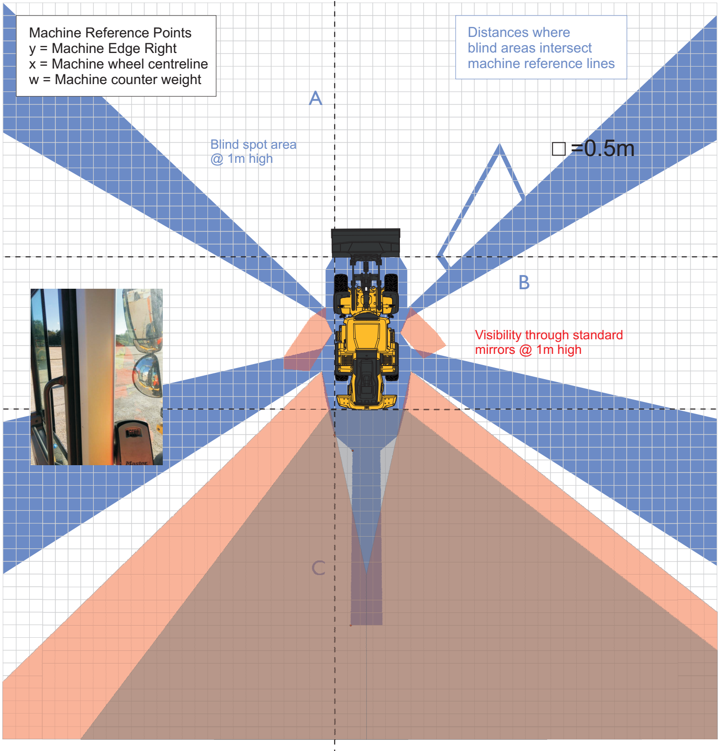
Volvo L60H
