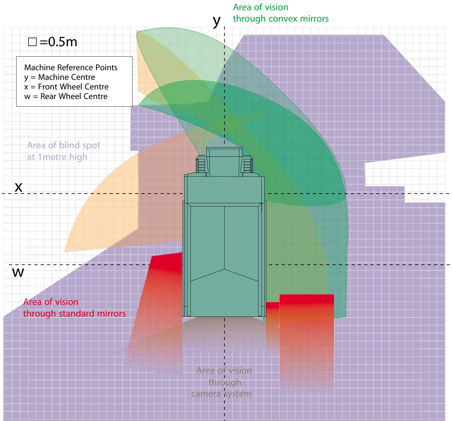
Terex TR100
