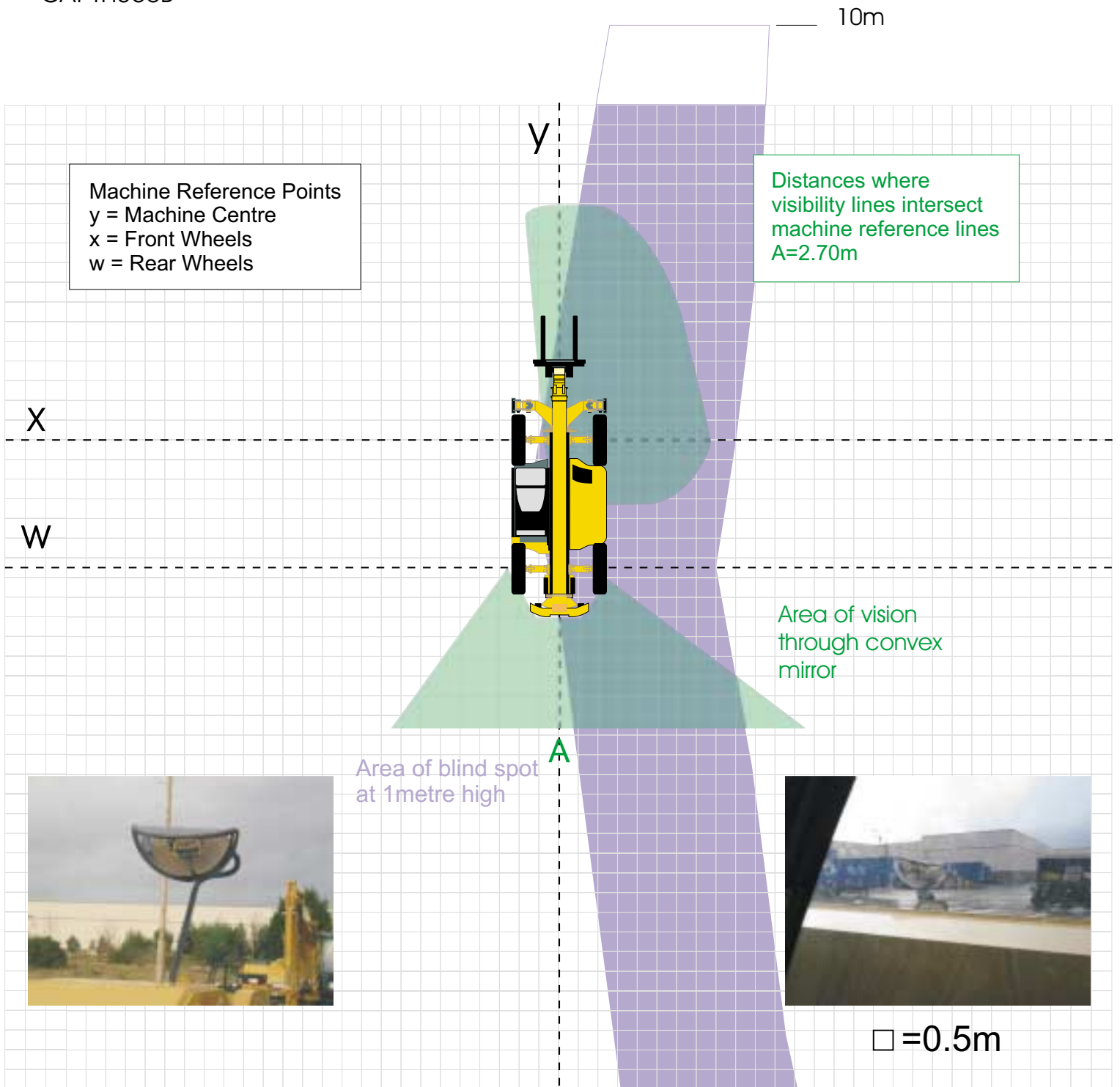
CAT TH360B
