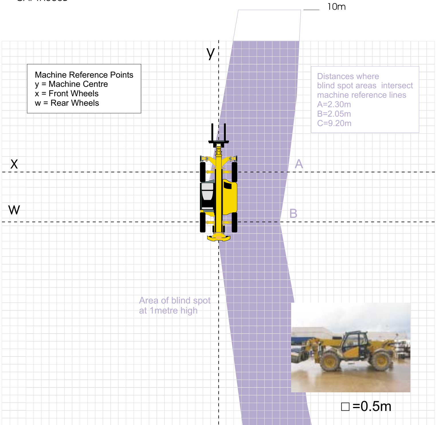
CAT TH360B
