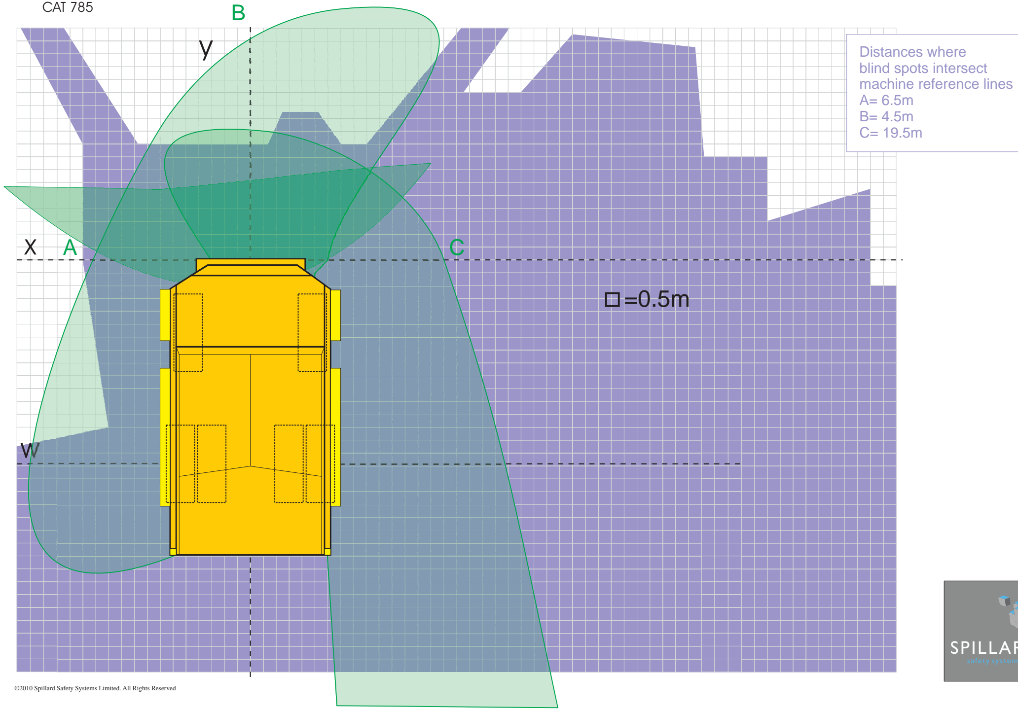
CAT 785
