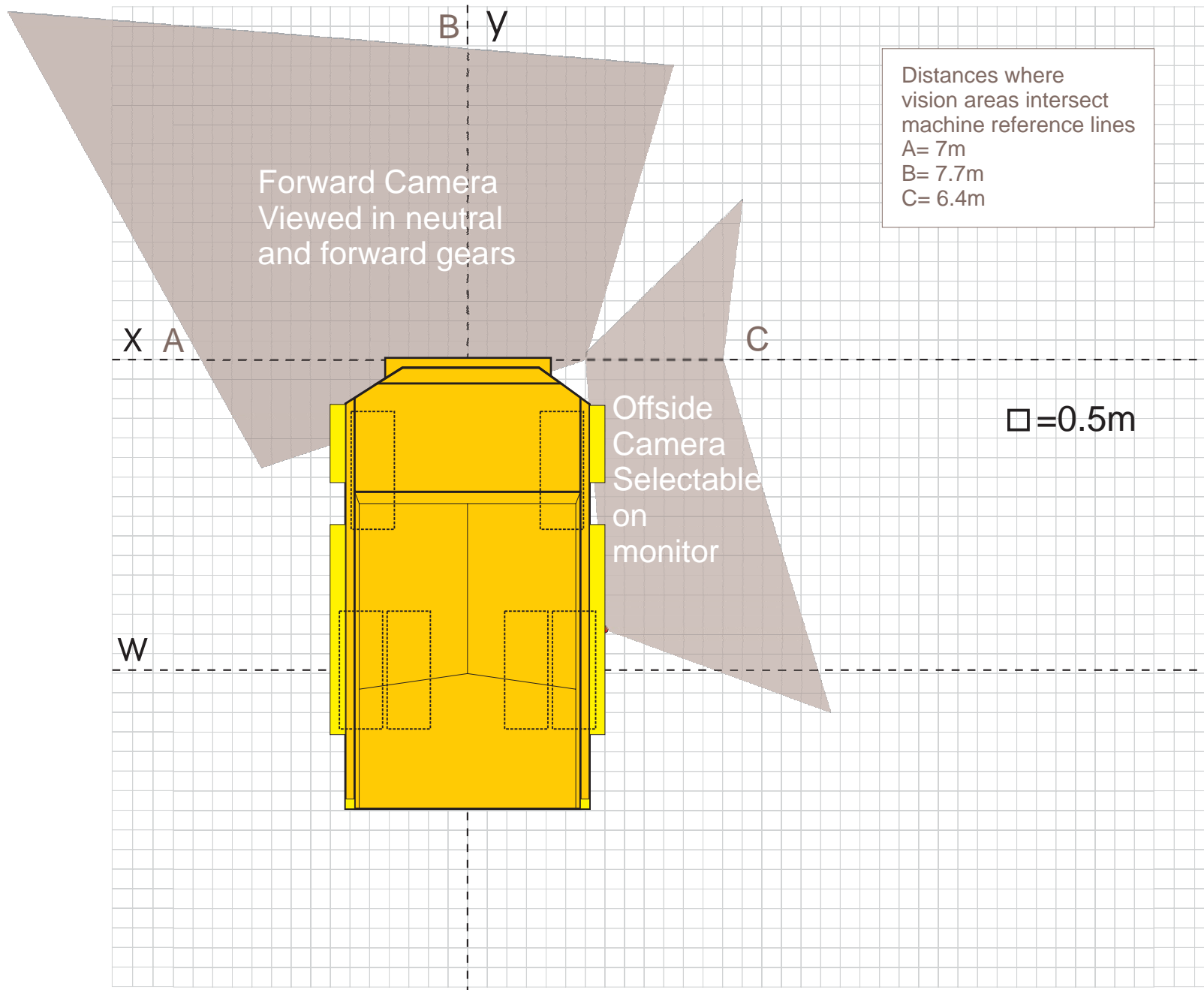
CAT 785
