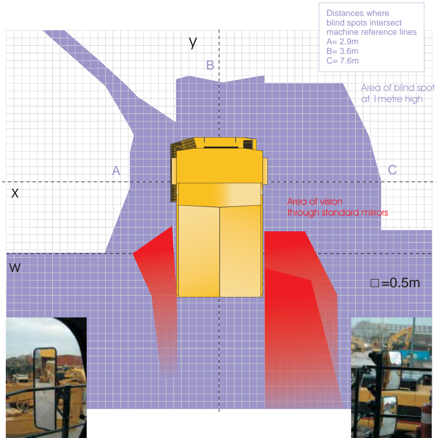
CAT 777F
